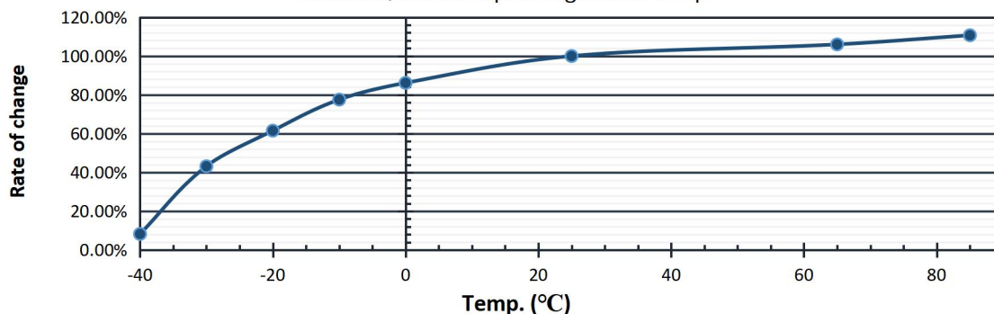
LIC1013Q3R8306 Cap. changes with Temp.
