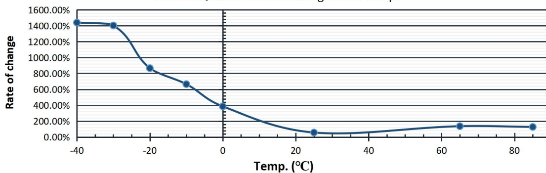
LIC1030Q3R8107 ESR DC changes with Temp.
