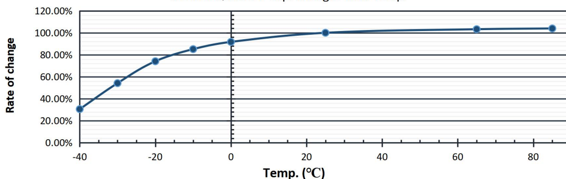
LIC1620Q3R8277 Cap. changes with Temp.
