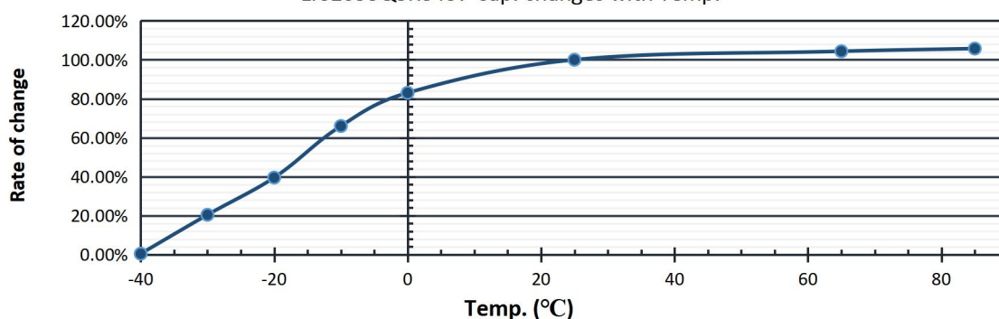
LIC1635Q3R8457 Cap. changes with Temp.
