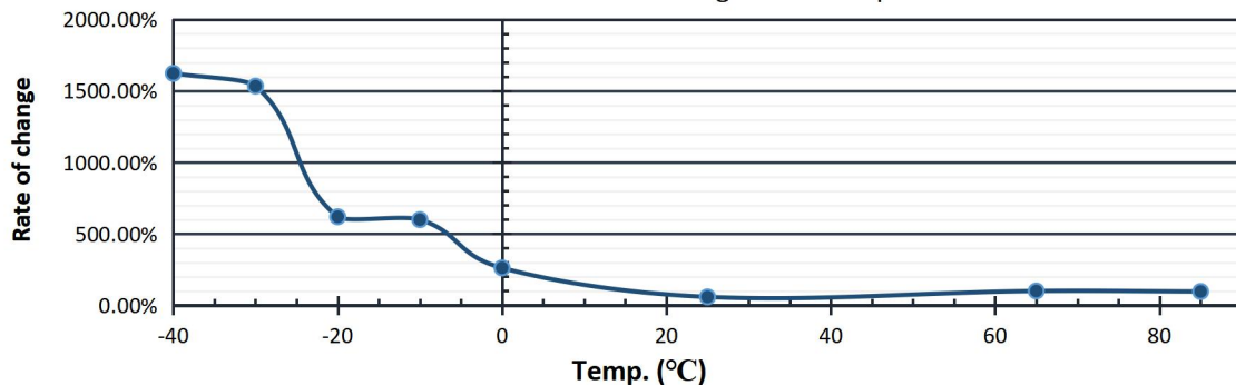
LIC1313Q3R8706 ESR DC changes with Temp.
