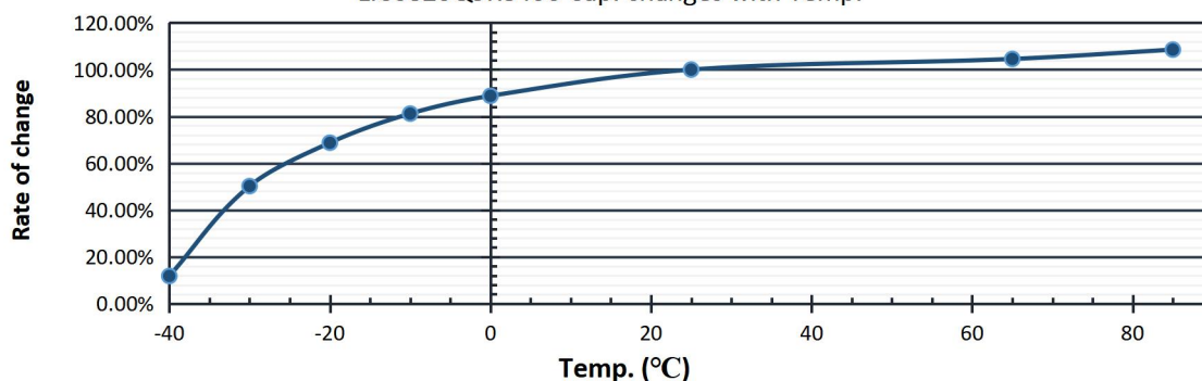
LIC0820Q3R8406 Cap. changes with Temp.
