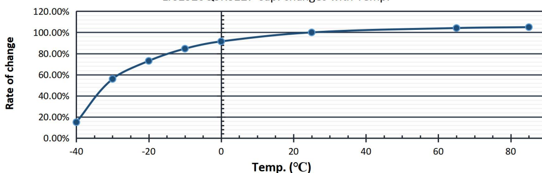
LIC1320Q3R8127 Cap. changes with Temp.
