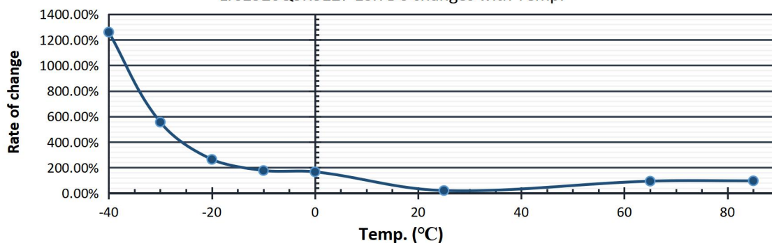
LIC1320Q3R8127 ESR DC changes with Temp.
