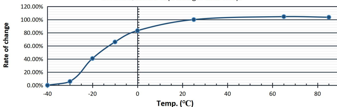
LIC1030Q3R8107 Cap. changes with Temp.
