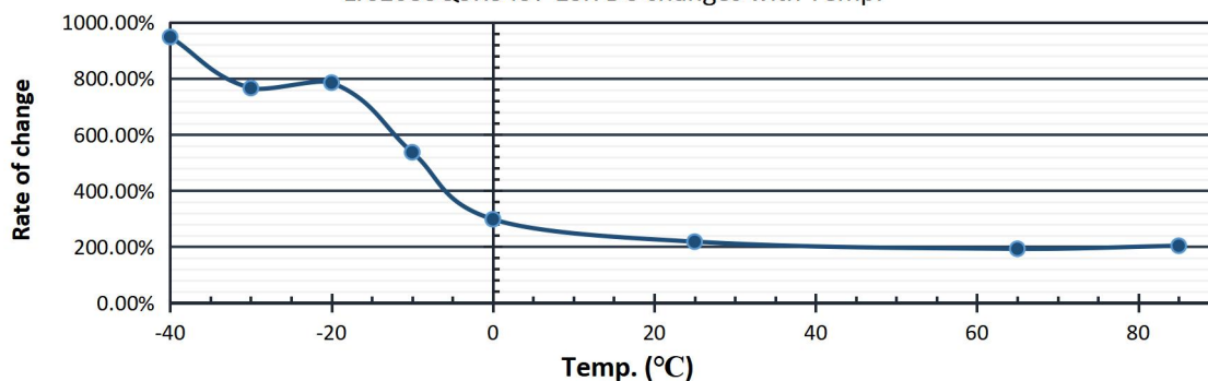
LIC1635Q3R8457 ESR DC changes with Temp.
