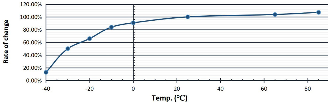
LIC0825Q3R8506 Cap. changes with Temp.
