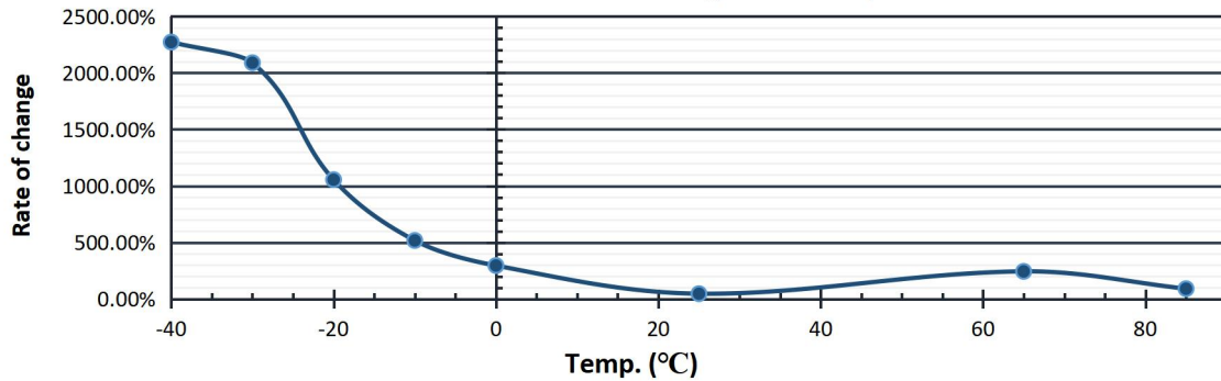
LIC0825Q3R8506 ESR DC changes with Temp.
