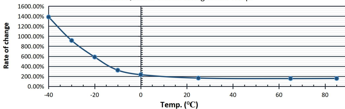
LIC1620Q3R8277 ESR DC changes with Temp.
