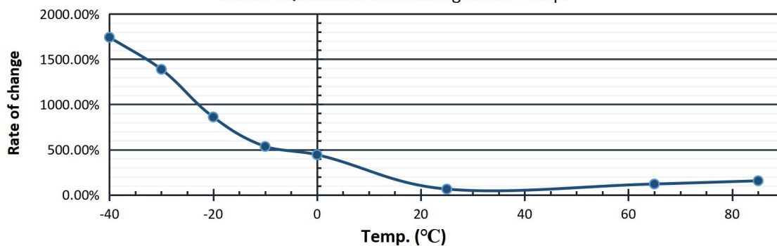
LIC1013Q3R8306 ESR DC changes with Temp.
