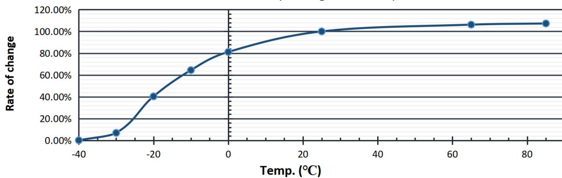
LIC1313Q3R8706 Cap. changes with Temp.
