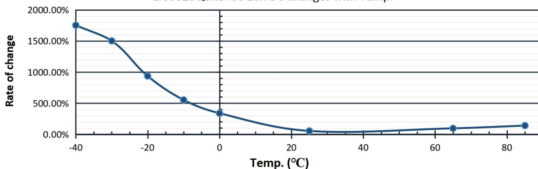
LIC0820Q3R8406 ESR DC changes with Temp.
